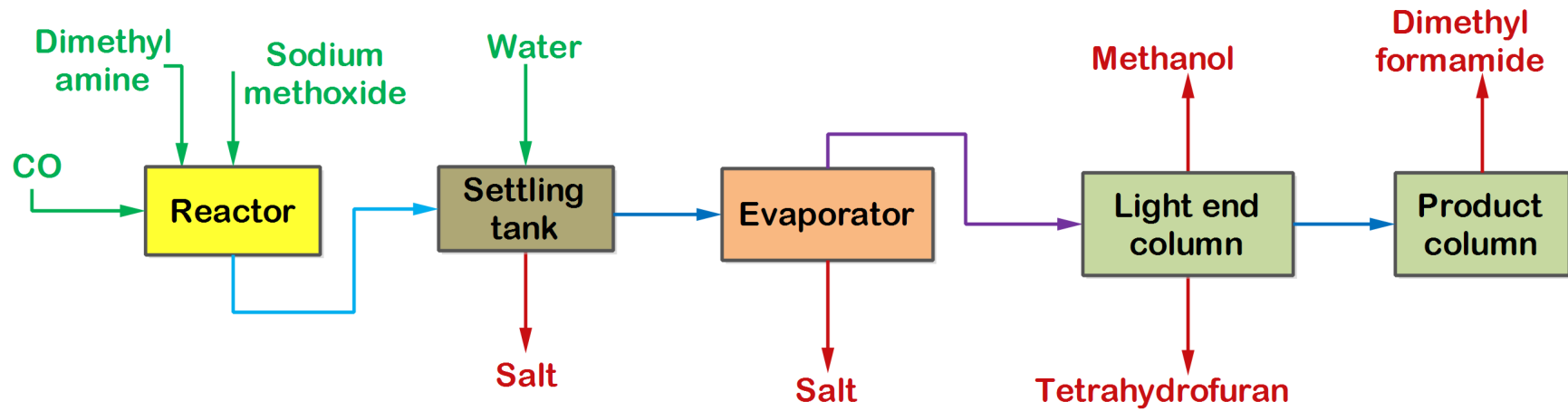
Figure: Manufacture of dimethyl formamide from methyl amine
